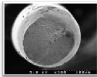
Annealed 316 LVM under tension 1
